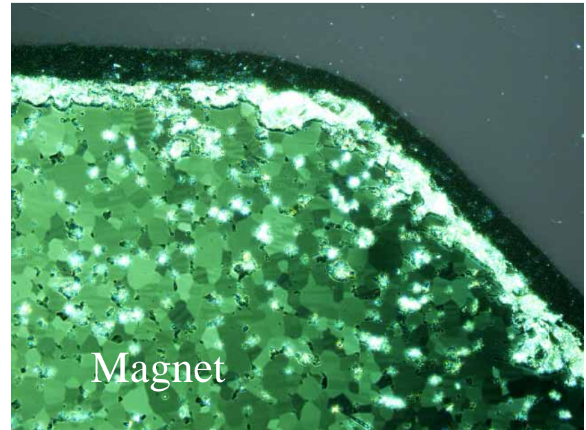
Coating
